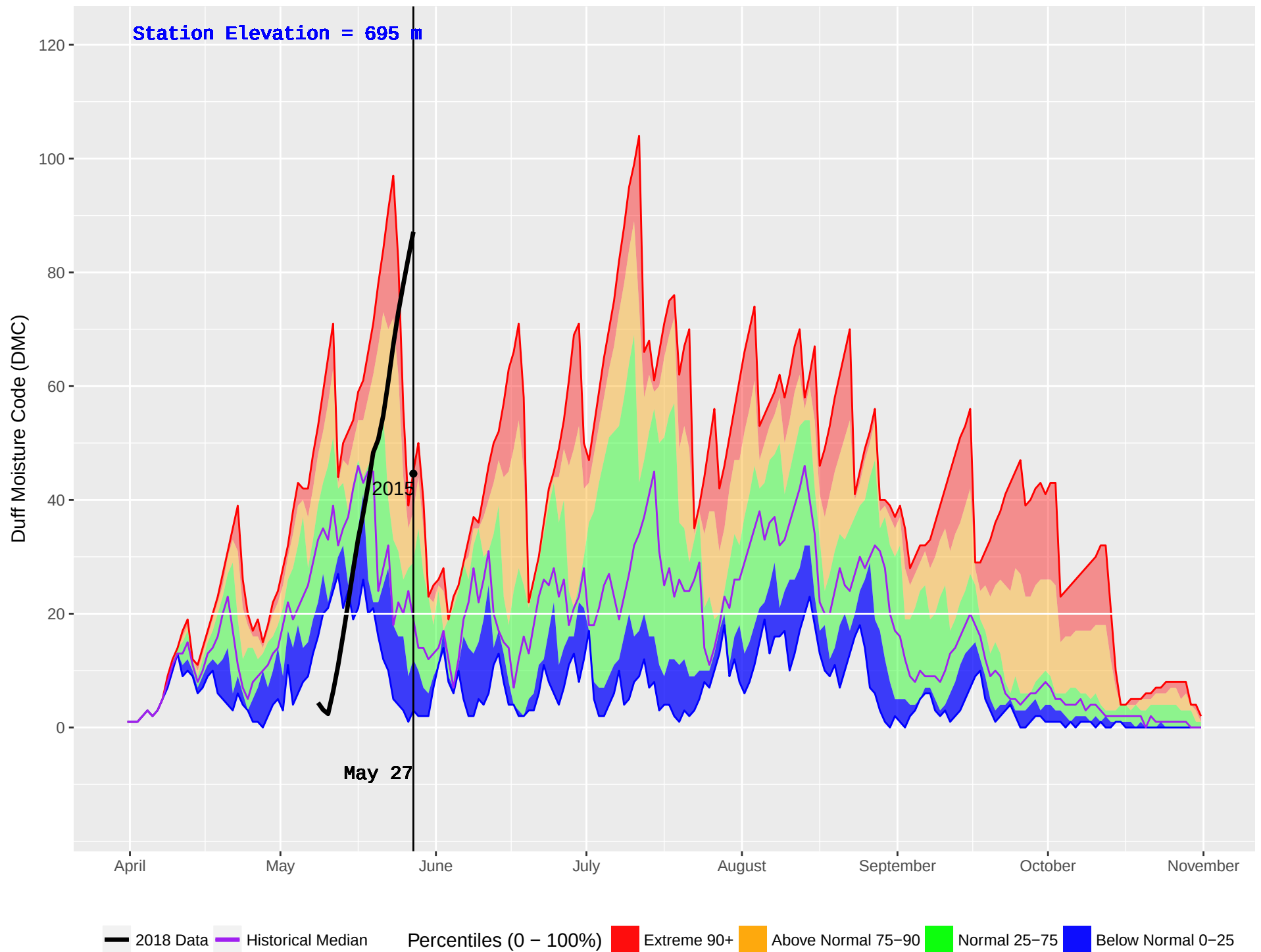
BLUE RIVER 2 (1108) : Historical (2011–2016) and Current (2018) Noon Duff Moisture Code (DMC)
