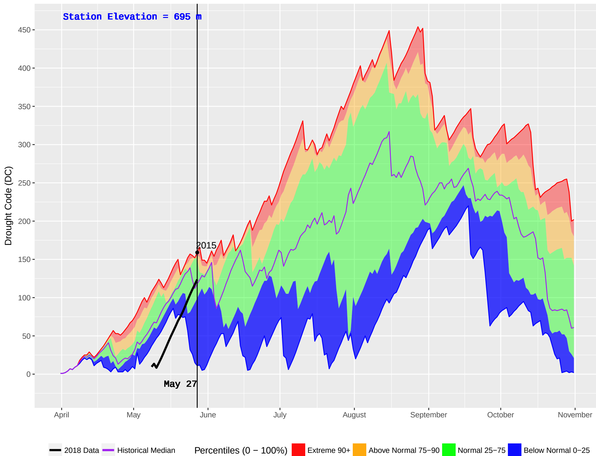
BLUE RIVER 2 (1108) : Historical (2011–2016) and Current (2018) Noon Drought Code (DC)
