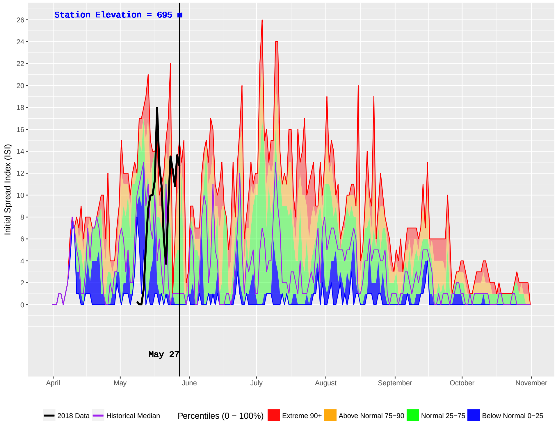
BLUE RIVER 2 (1108) : Historical (2011–2016) and Current (2018) Noon Initial Spread Index (ISI)
