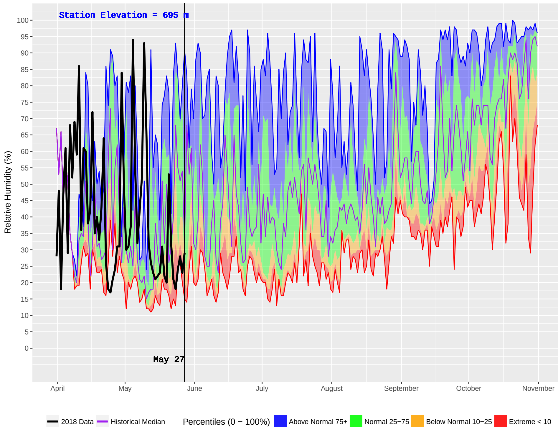
BLUE RIVER 2 (1108) : Historical (2011–2016) and Current (2018) Noon Relative Humidity
