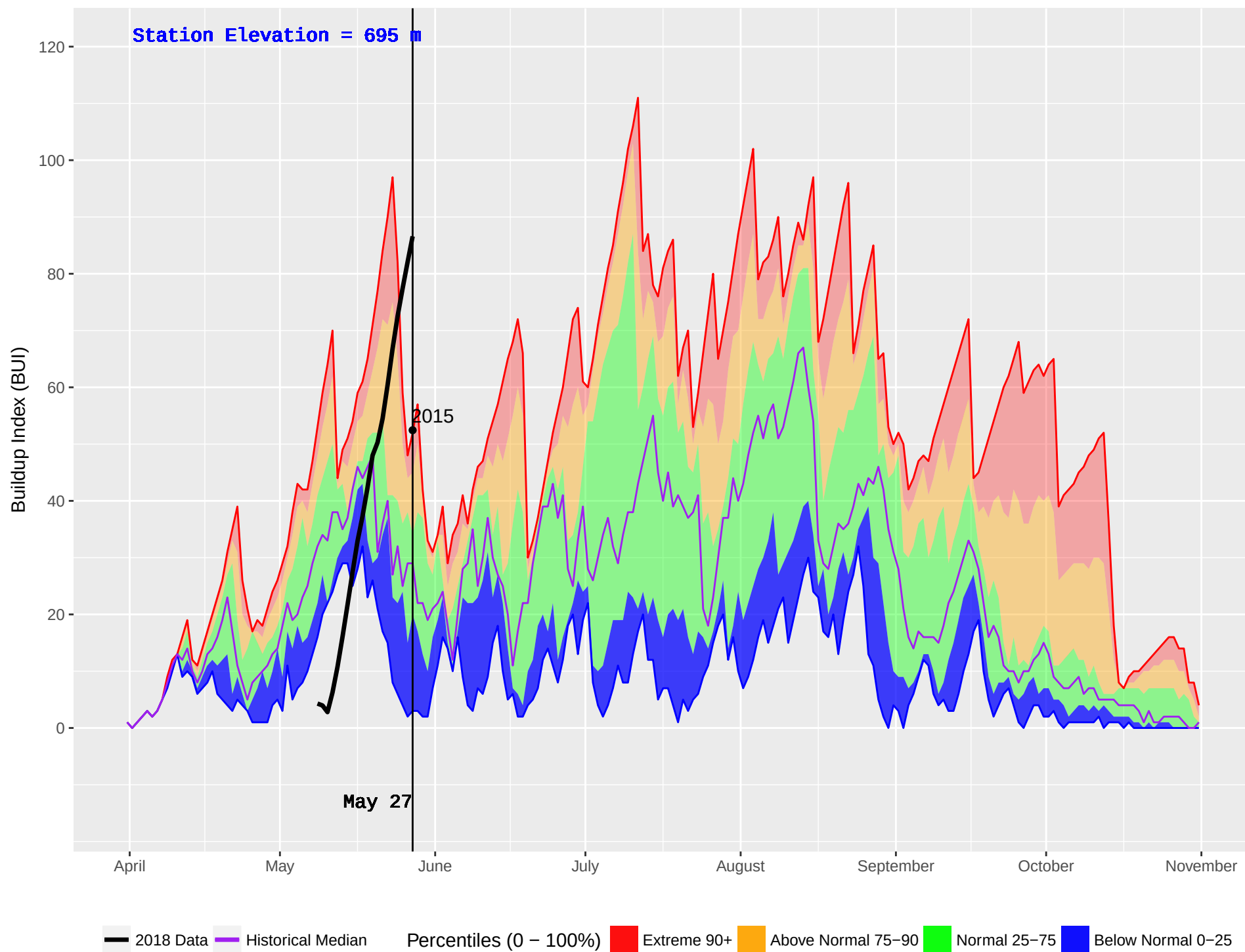
BLUE RIVER 2 (1108) : Historical (2011–2016) and Current (2018) Noon Buildup Index (BUI)
