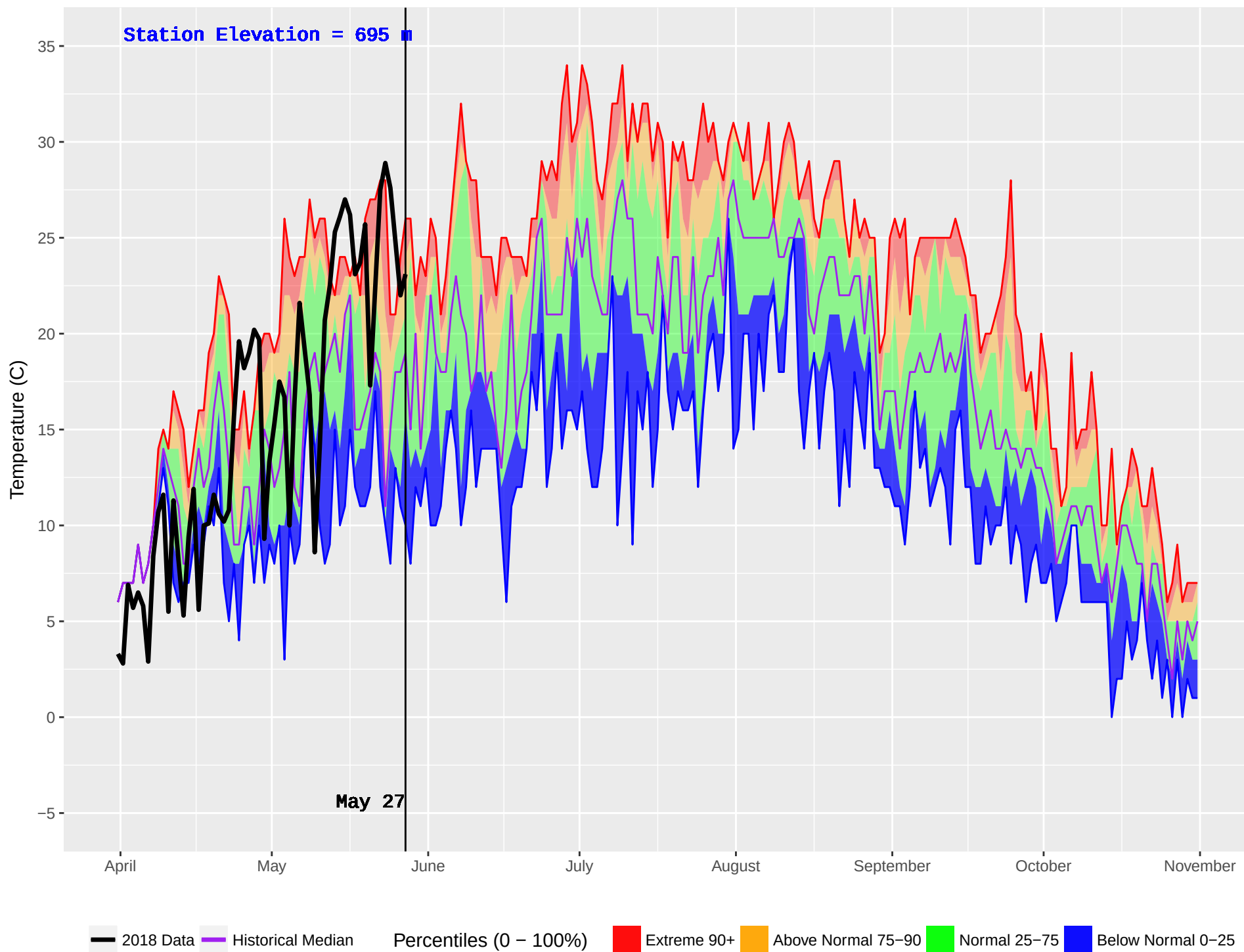
BLUE RIVER 2 (1108) : Historical (2011–2016) and Current (2018) Noon Temperature
